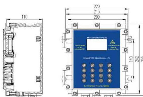
Explosion-proof Transmitter
