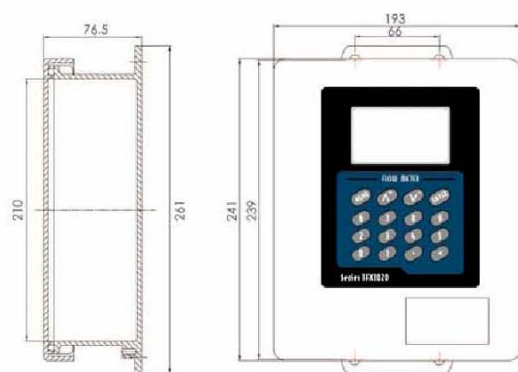
Standard Transmitter
